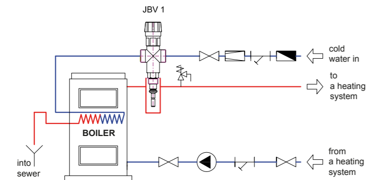
Fig. 4: Piping diagram for JBV1 with a non-return valve used
