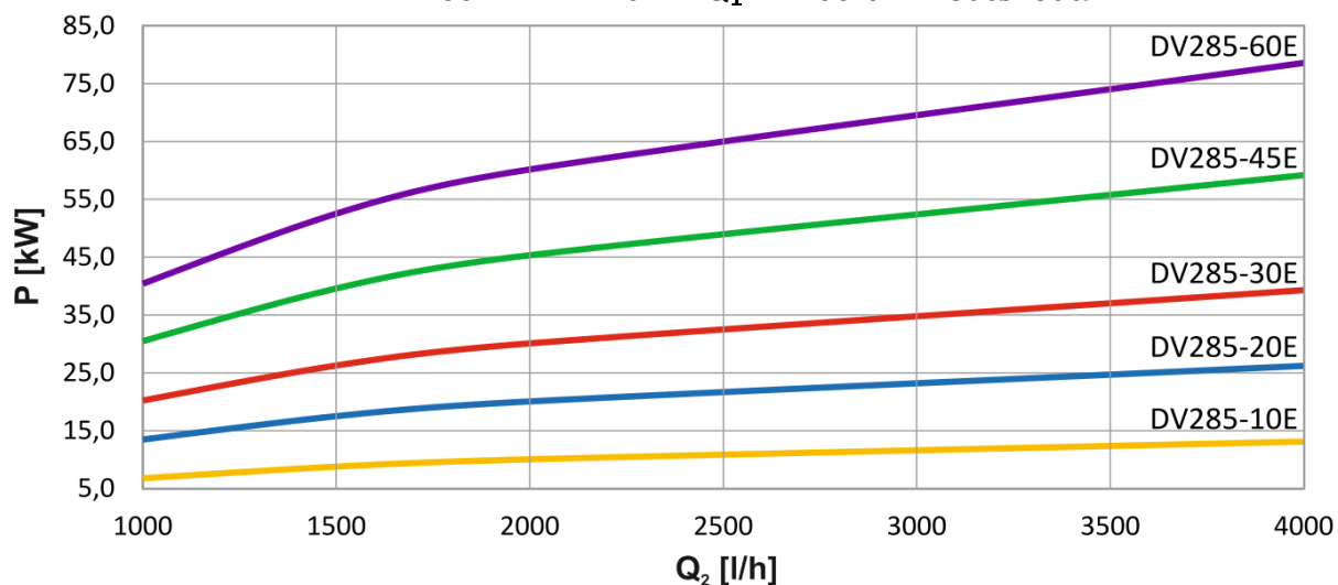
DV285E - \Delta T = 10 K - Q_1 = 2400 l/h - voda/voda
