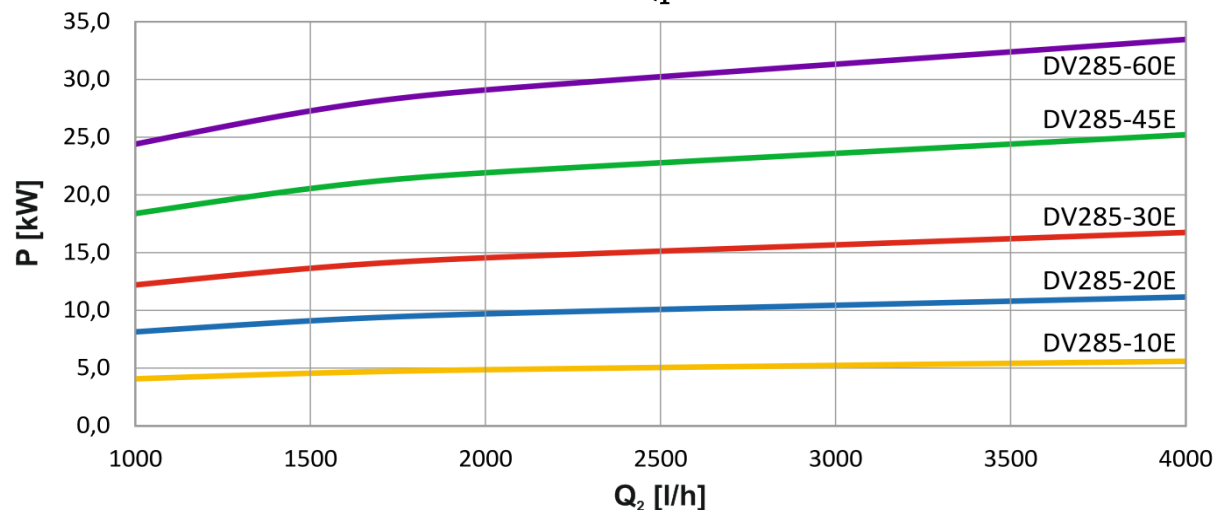
DV285E - \Delta T = 6 \text{ K} - Q_1 = 2400 \text{ l/h} - voda/voda
