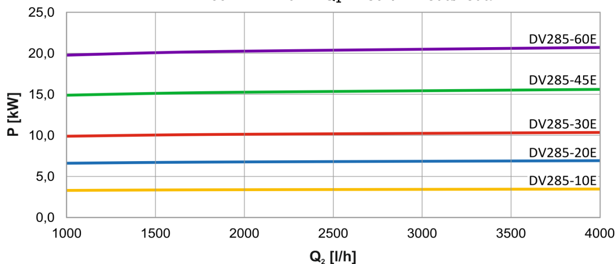
DV285E - \Delta T = 6 \text{ K} - Q_1 = 1500 \text{ l/h} - voda/voda
