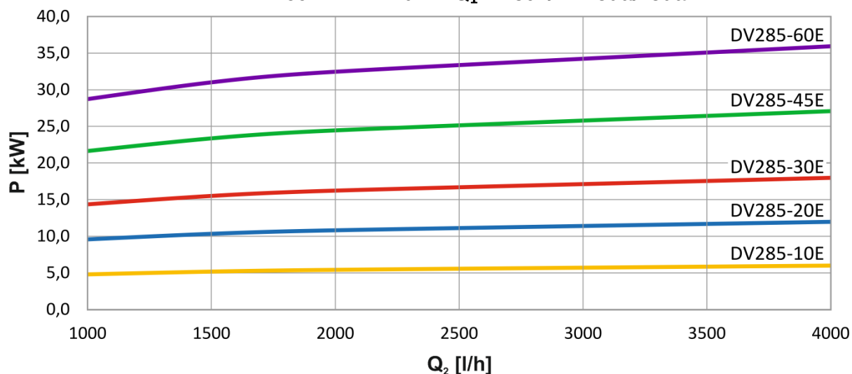
DV285E - \Delta T = 10 K - Q_1 = 1500 l/h - voda/voda
